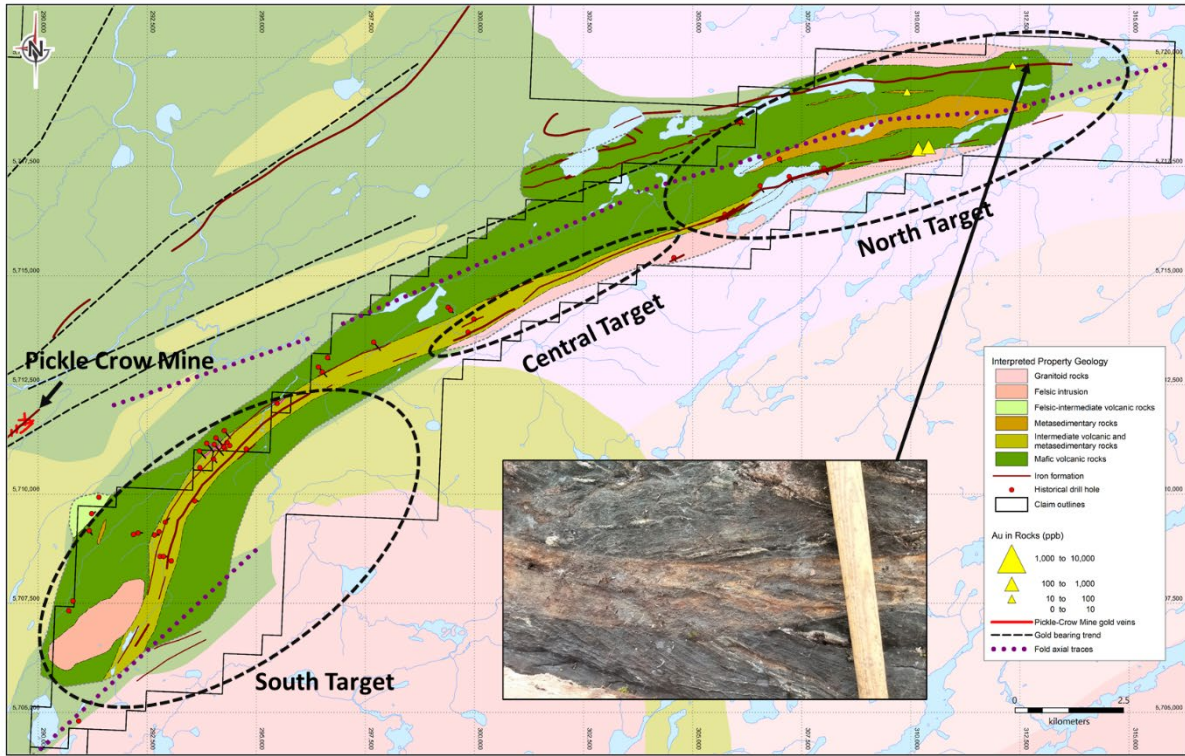
Figure 1: Interpreted Geology
