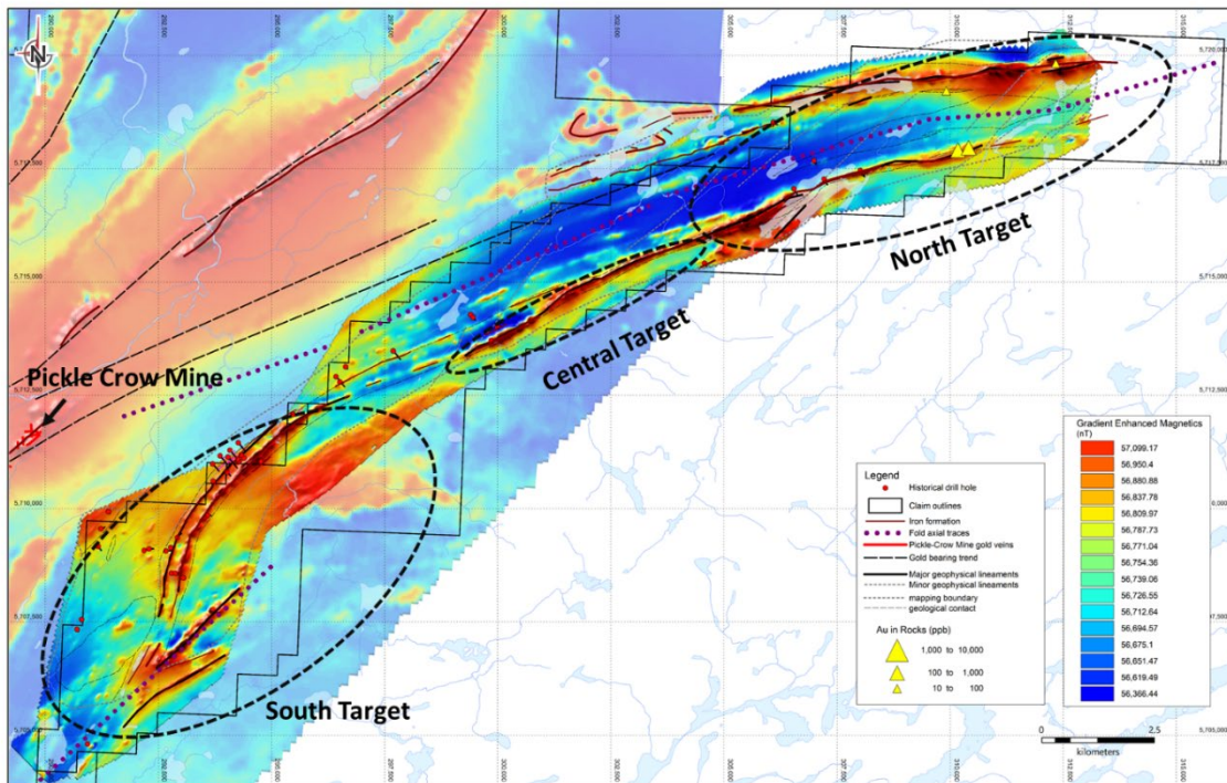
Figure 2: Total Field Magnetics with Interpreted Structure
