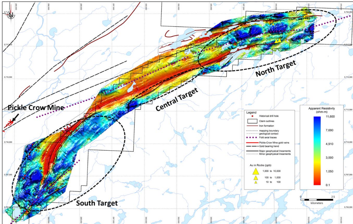
Figure 3: Apparent Resistivity with Interpreted Structure
