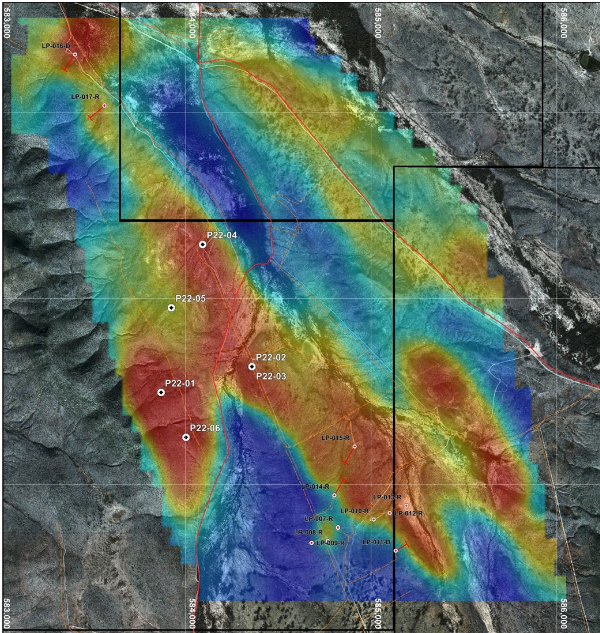
Figure 1: Drill plan with 100 metre depth slice of Chargeability
