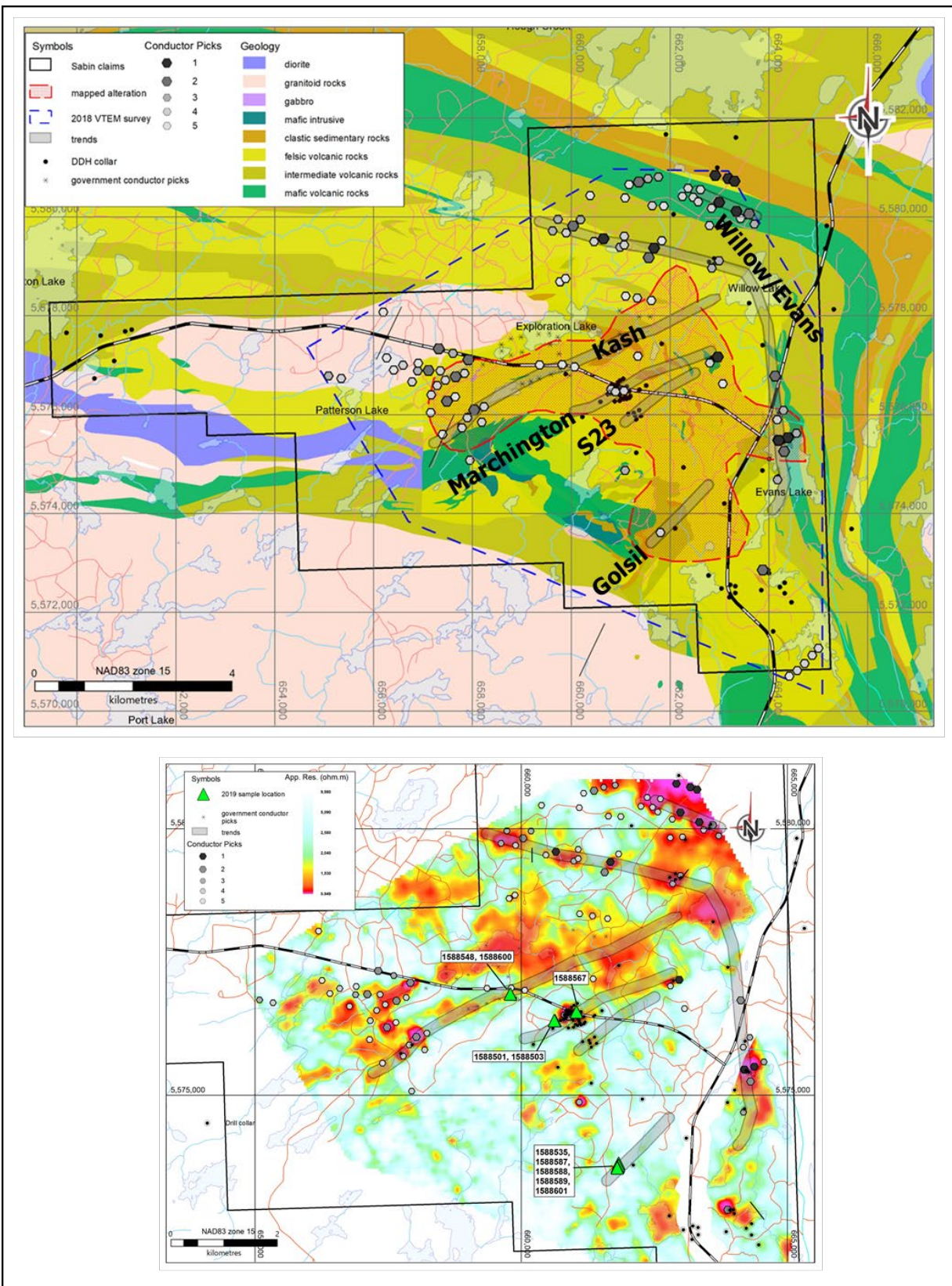
Figure 1: Sabin geology with Conductors; detail-Sabin samples on apparent resistivity
