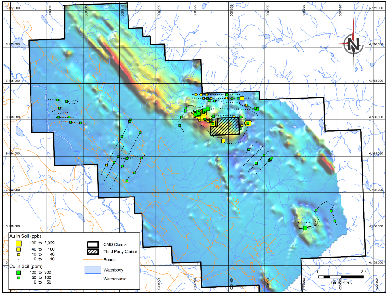
Figure 2: Magnetic Survey
